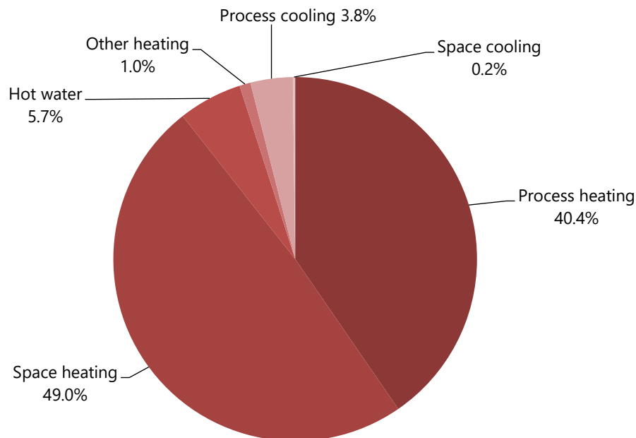
Figure A1-13: Heat demand by end use across all sectors in the Netherlands in 2015. (Heat Roadmap Europe, 2017)
