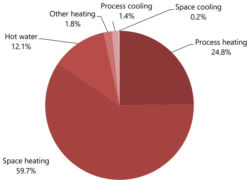
Figure A1-17: UK Heat and cooling demand by end use across all sectors in the UK 2015 (Heat Roadmap Europe, 2017)
