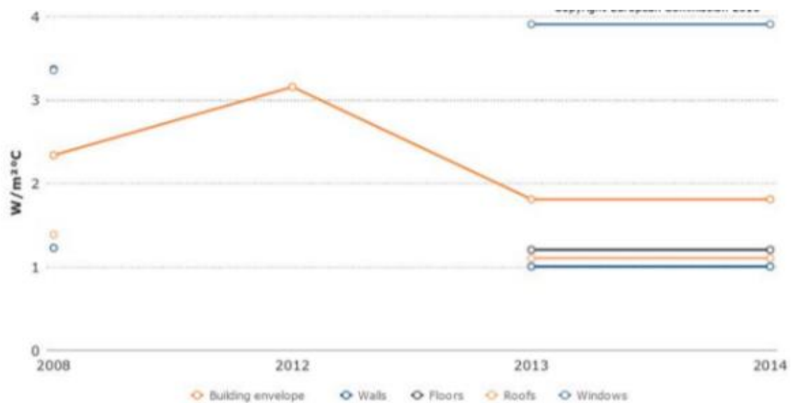
Figure A1-27: U- Values of building elements in the UK compared to the EU average (EU Building Stock Observatory, 2016d)
